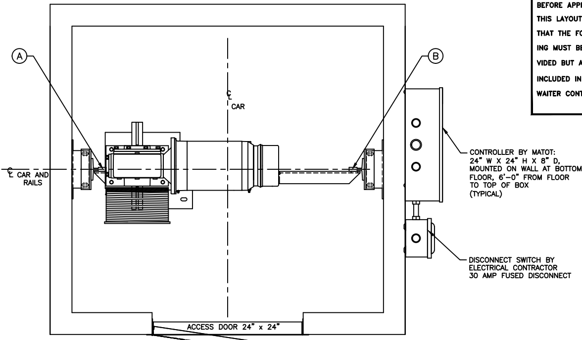
MACHINE PLAN SCALED: NONE
