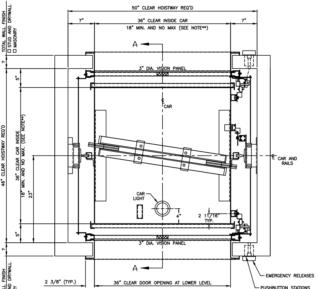
COMPOSITE FLOOR PLAN SCALED: NONE
