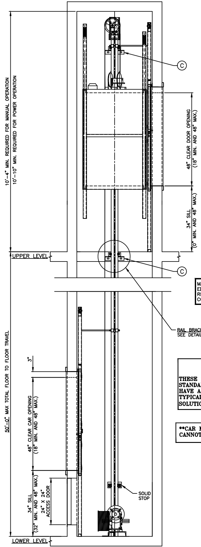
VIEW A-A, ELEVATION SCALED: NONE
