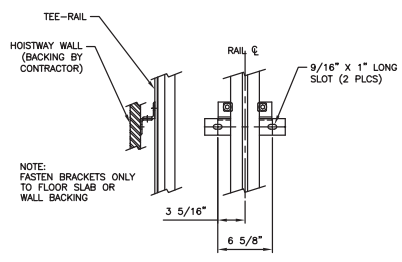
DETAIL B RAIL BRACKET ASSEMBLY
